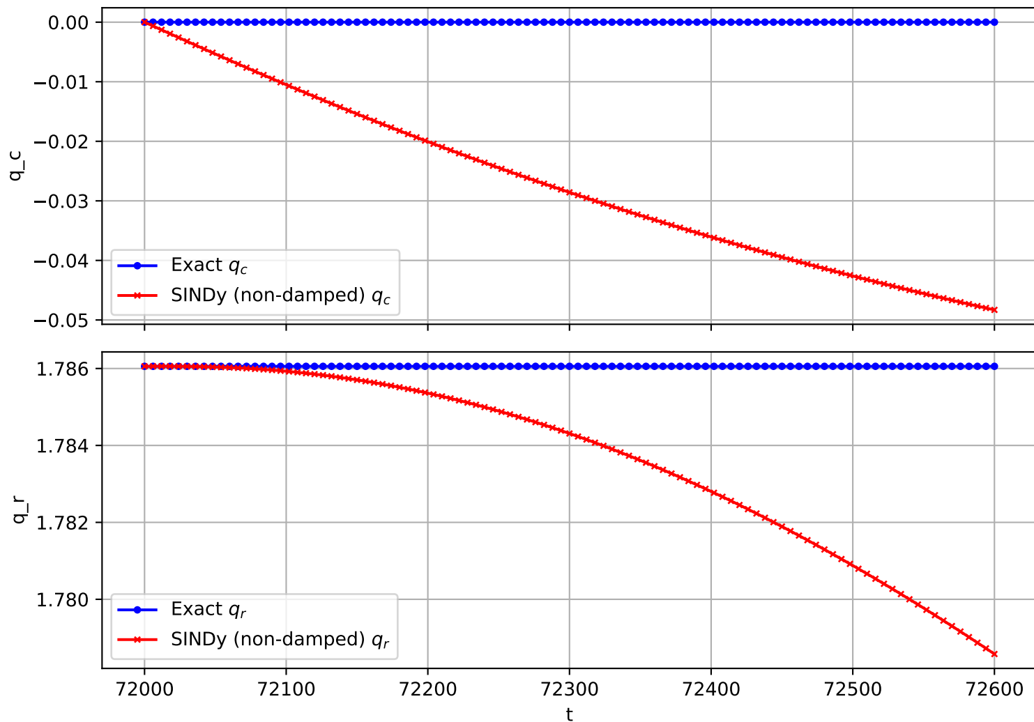
Trajectory 612 (non-damped)
