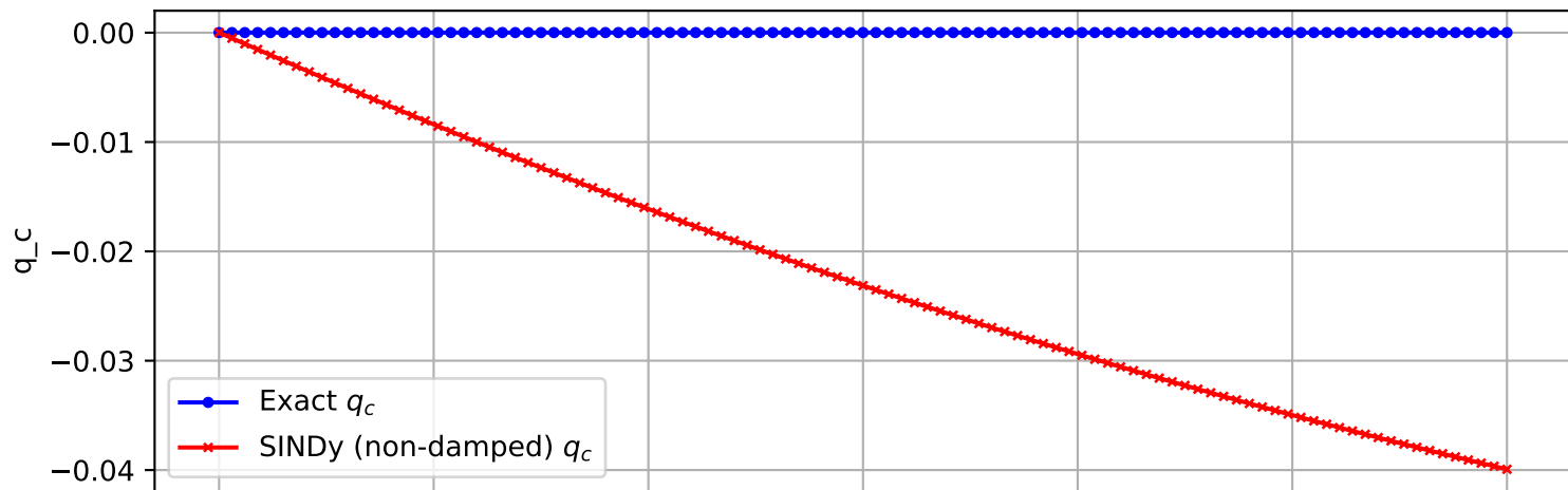
Trajectory 614 (non-damped)
