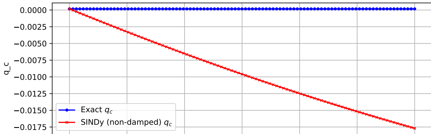
Trajectory 622 (non-damped)
