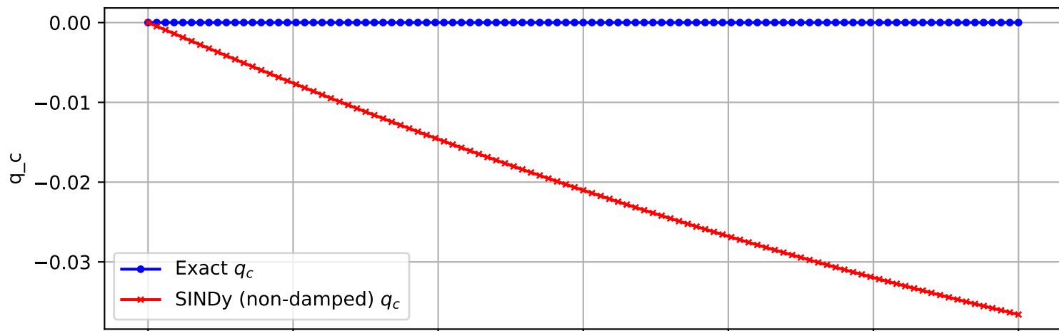
Trajectory 628 (non-damped)
