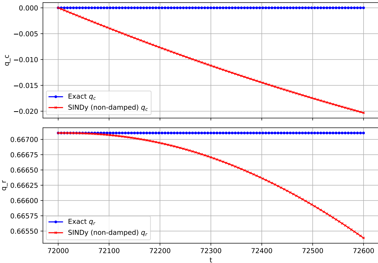
Trajectory 631 (non-damped)
