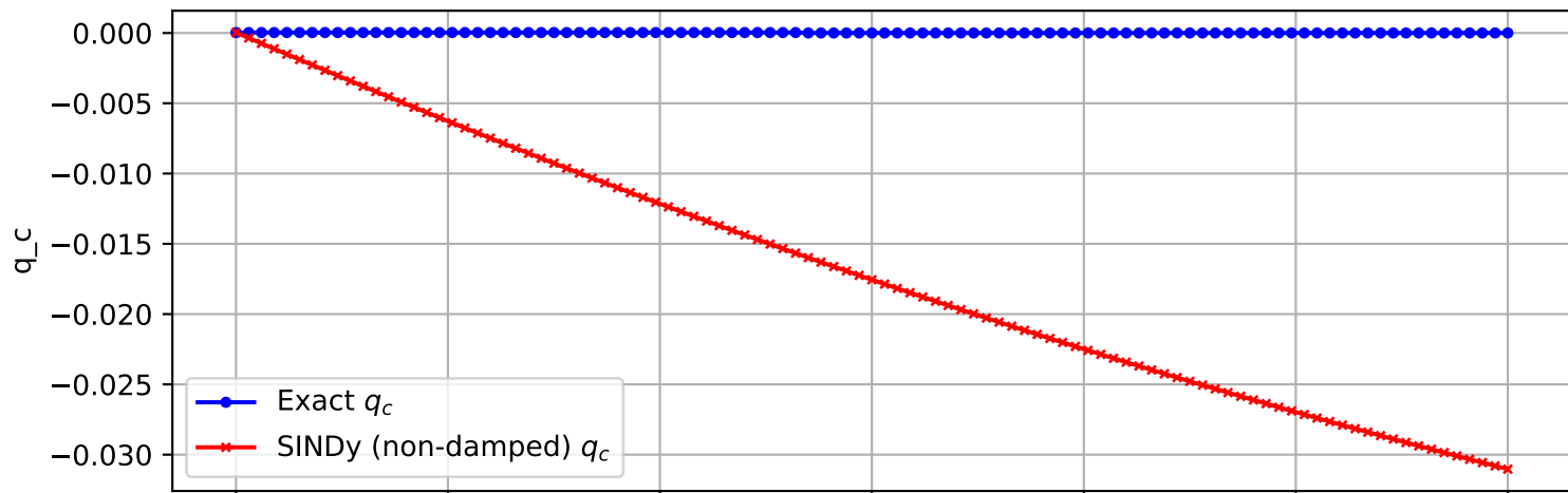
Trajectory 632 (non-damped)
