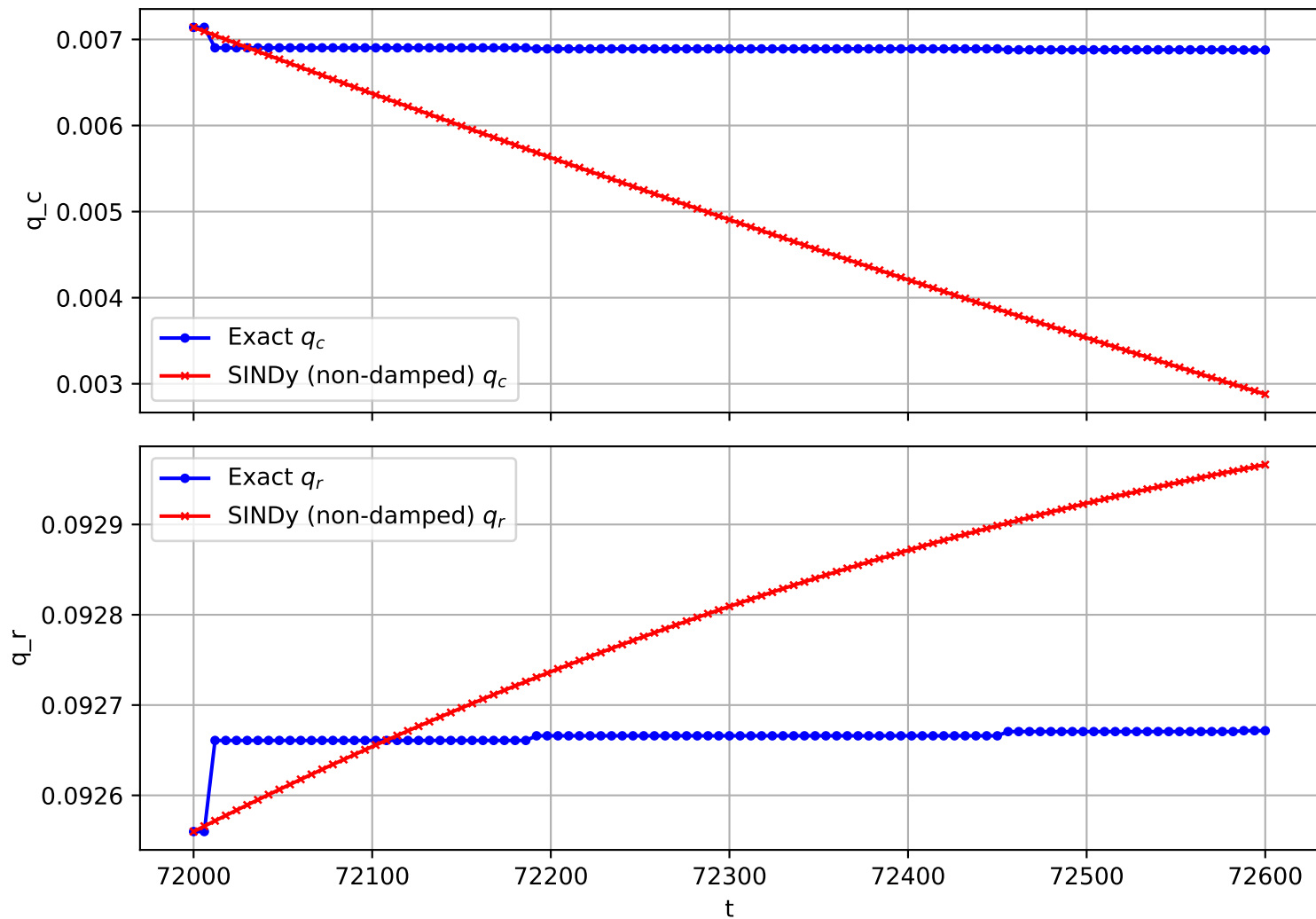
Trajectory 640 (non-damped)
