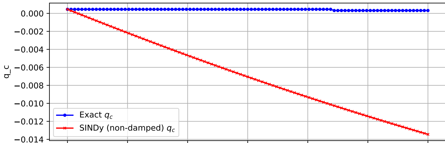
Trajectory 643 (non-damped)
