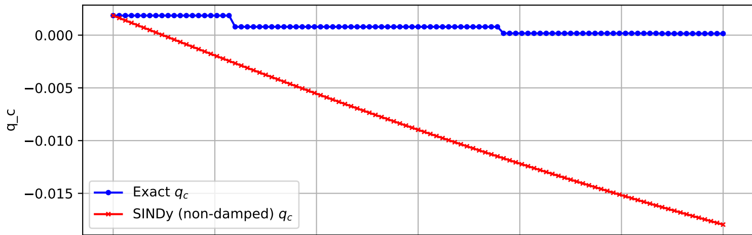
Trajectory 648 (non-damped)
