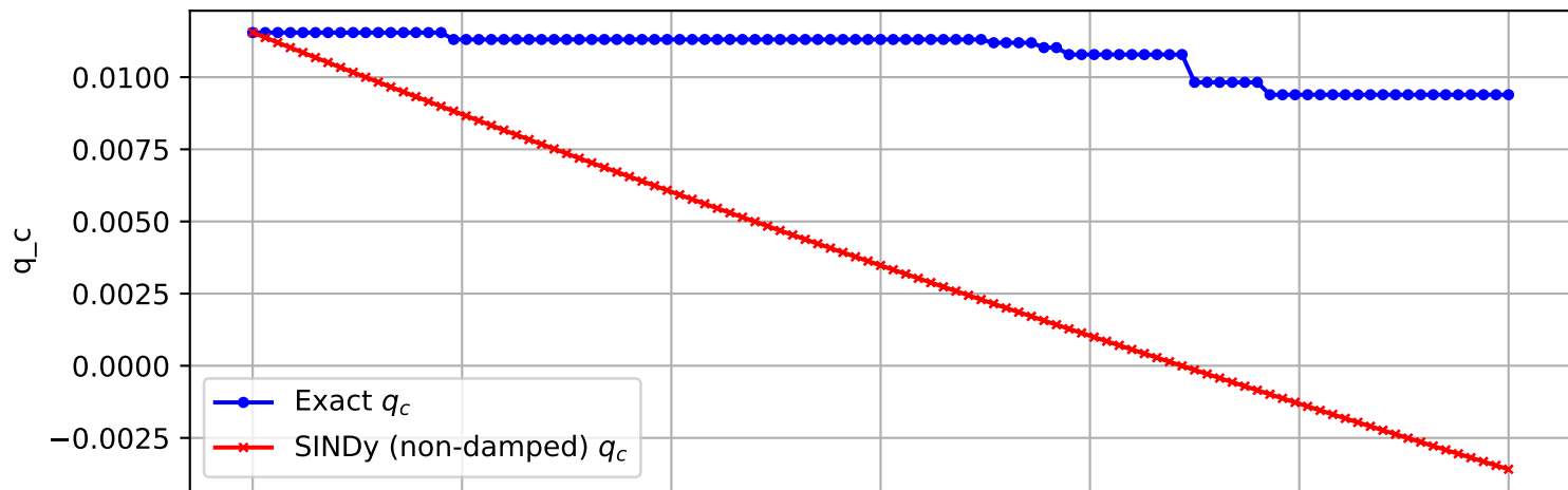
Trajectory 659 (non-damped)
