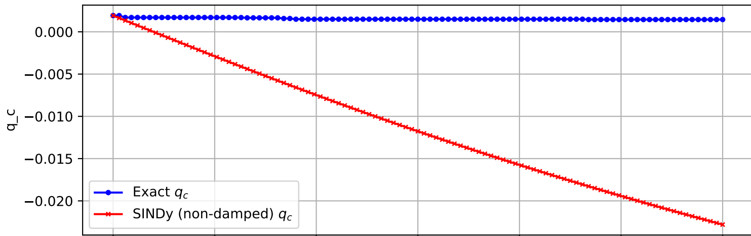
Trajectory 661 (non-damped)
