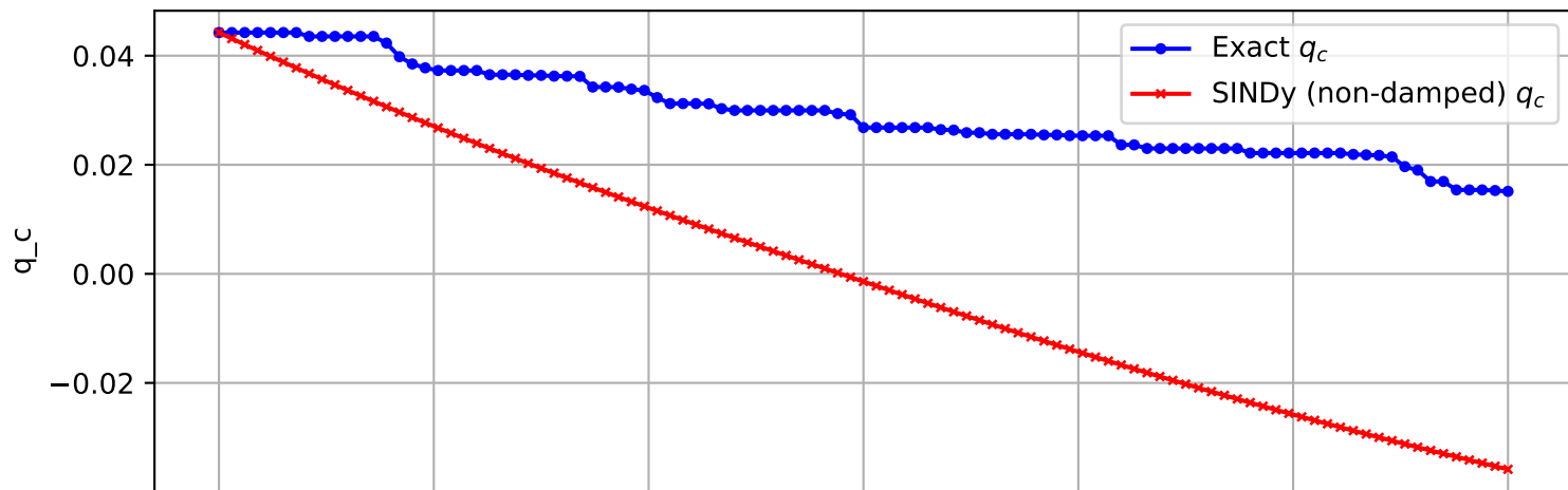
Trajectory 665 (non-damped)
