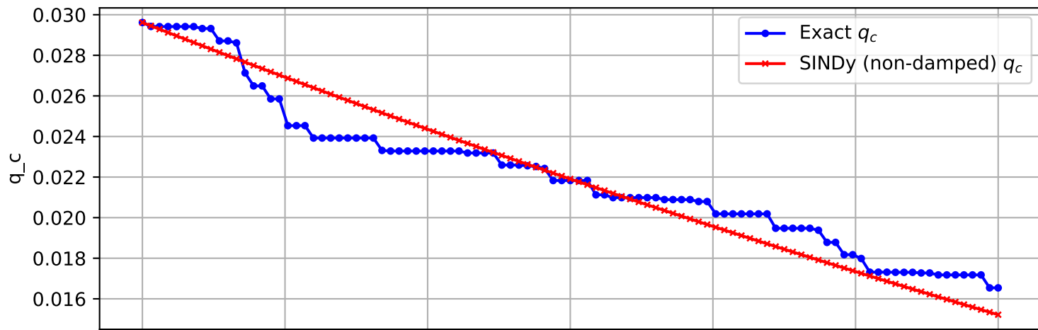
Trajectory 672 (non-damped)
