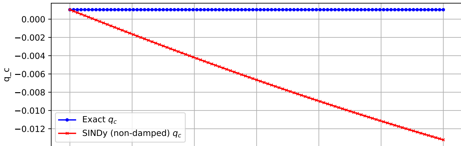
Trajectory 676 (non-damped)
