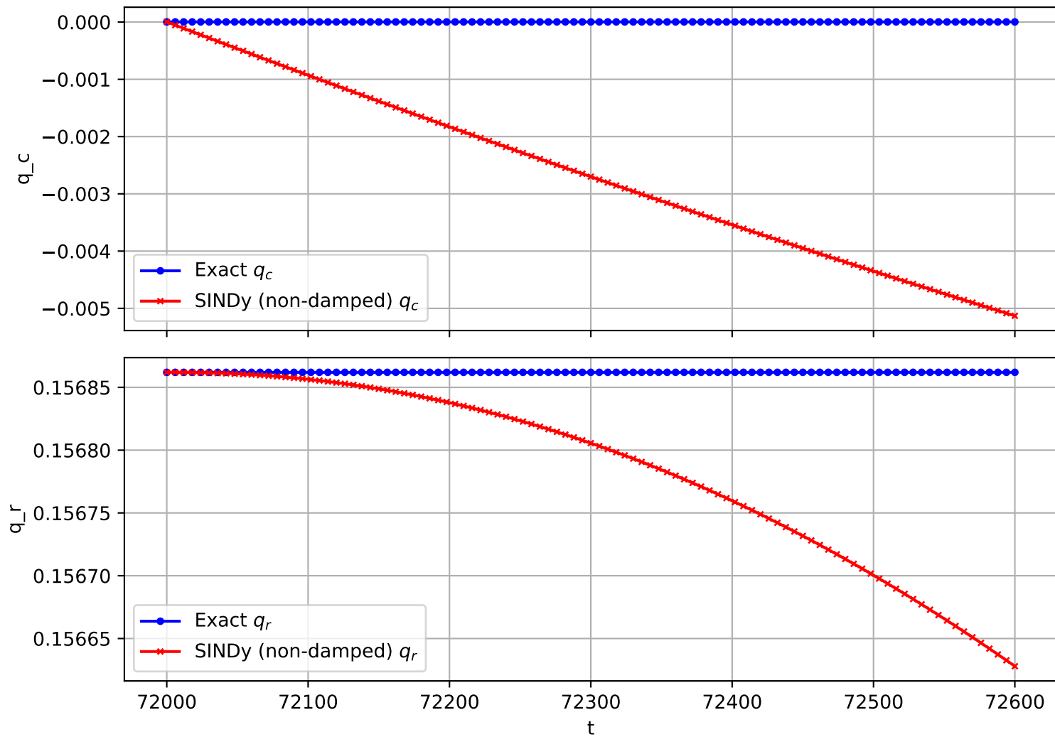
Trajectory 689 (non-damped)
