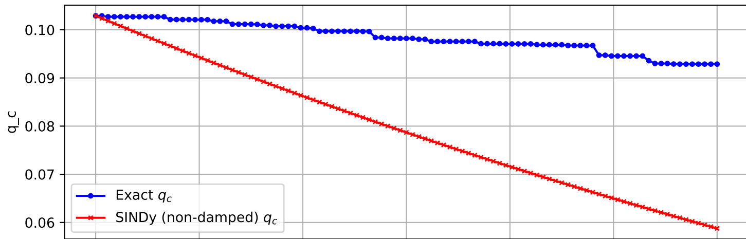
Trajectory 693 (non-damped)
