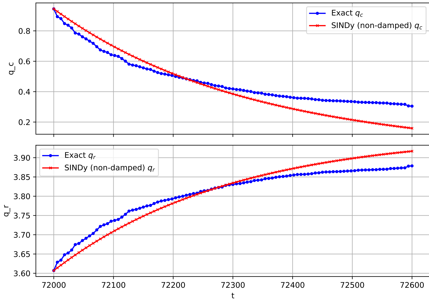
Trajectory 699 (non-damped)
