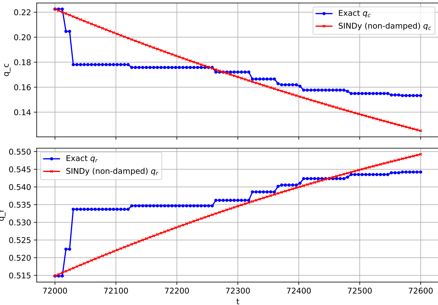
Trajectory 7 (non-damped)
