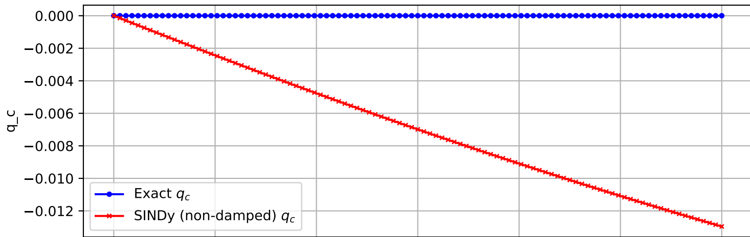
Trajectory 712 (non-damped)
