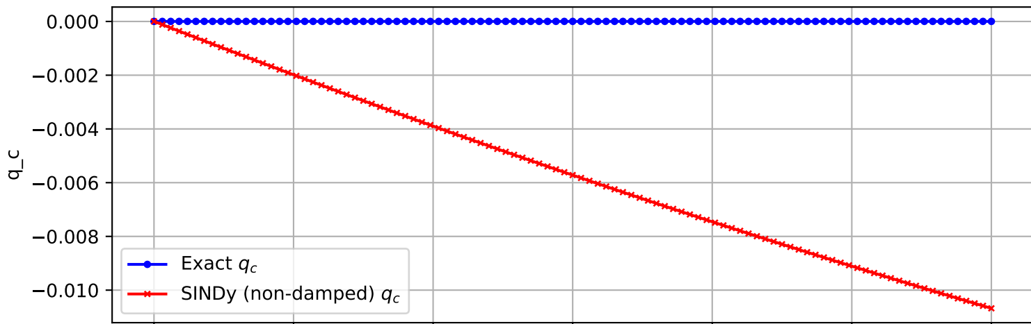
Trajectory 715 (non-damped)
