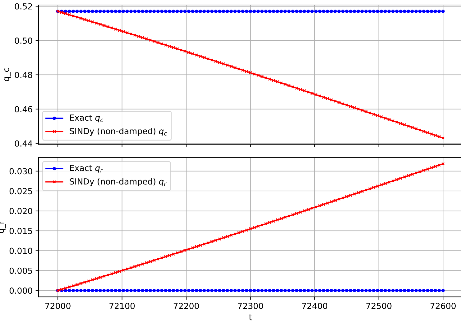
Trajectory 72 (non-damped)
