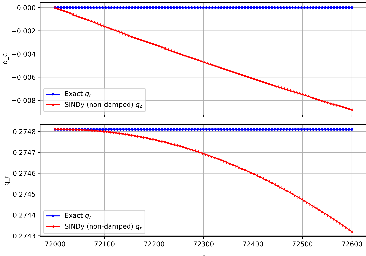
Trajectory 724 (non-damped)
