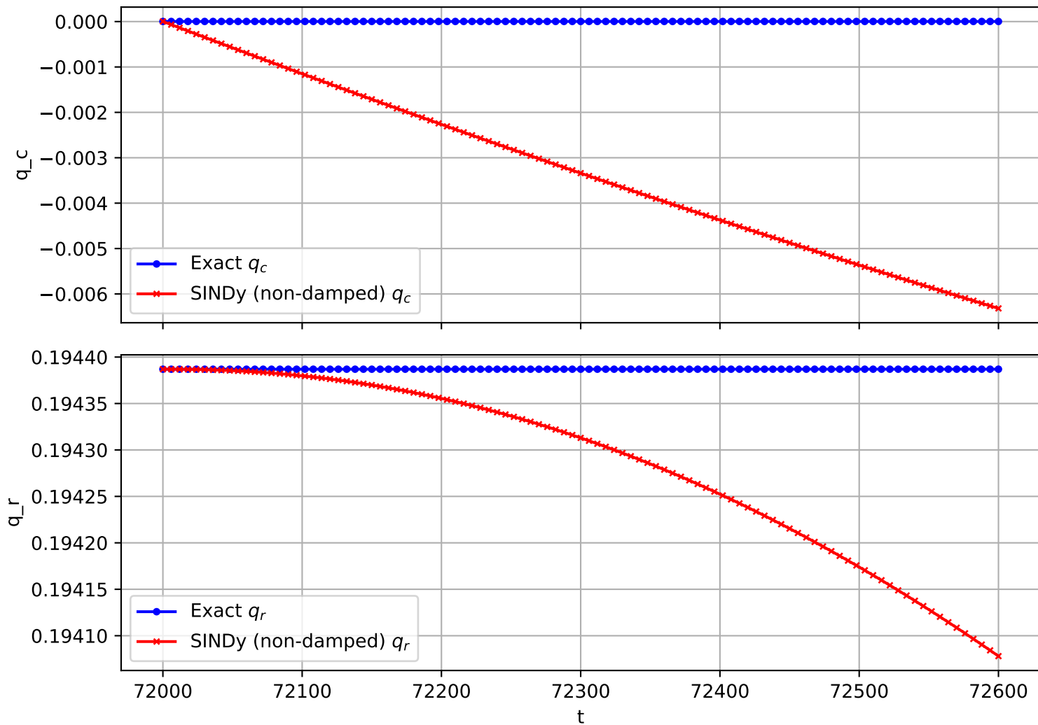
Trajectory 734 (non-damped)
