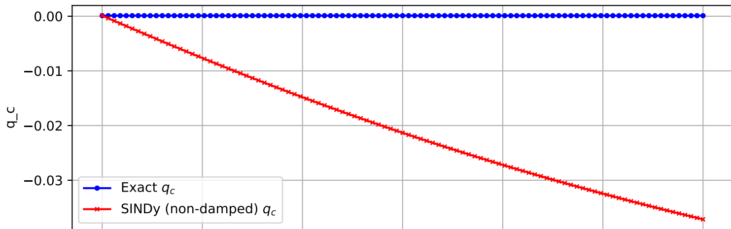
Trajectory 754 (non-damped)
