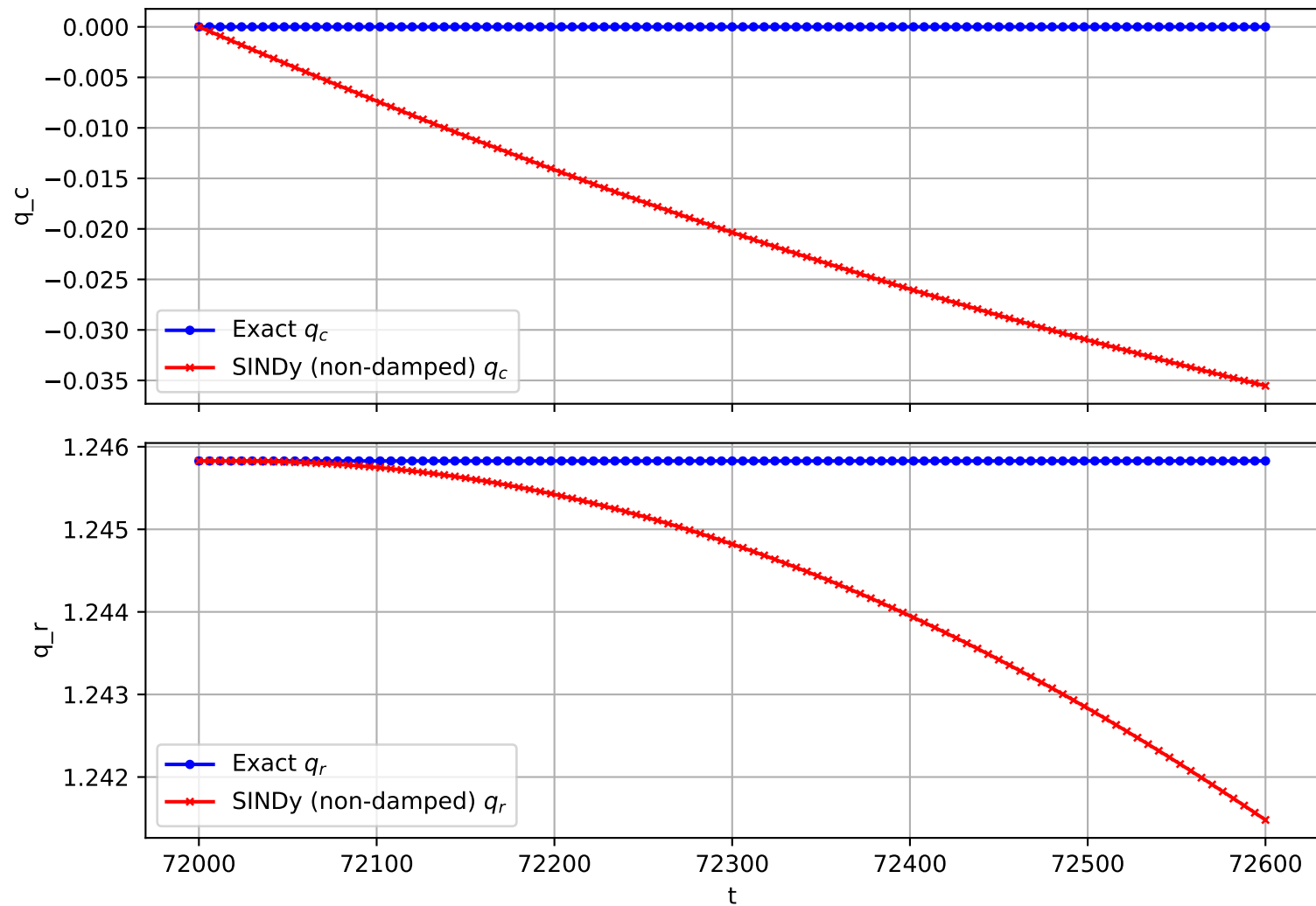
Trajectory 759 (non-damped)
