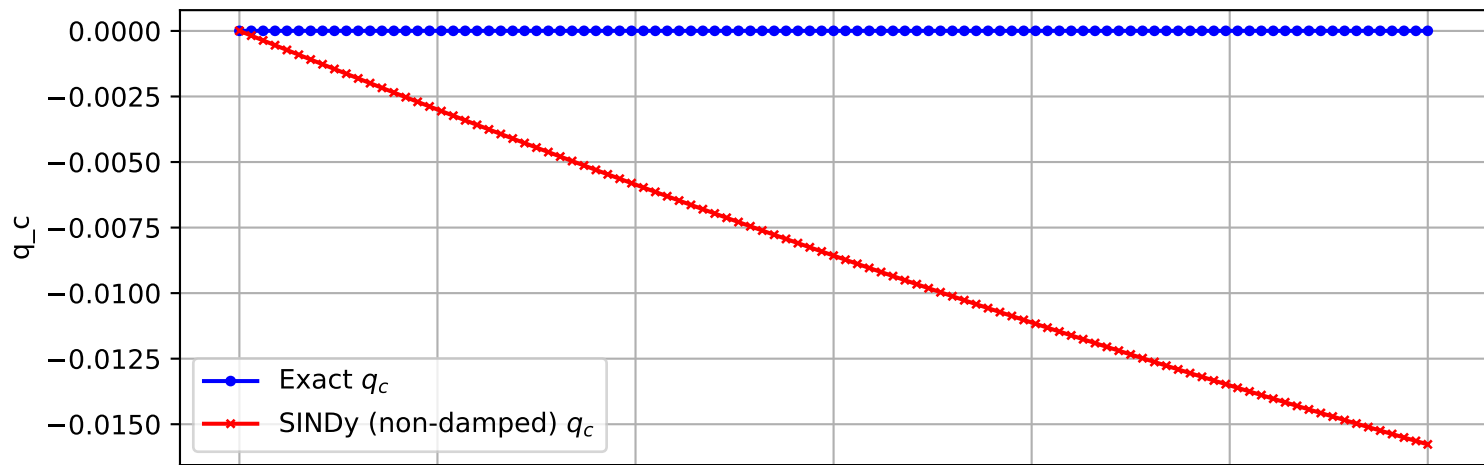
Trajectory 760 (non-damped)
