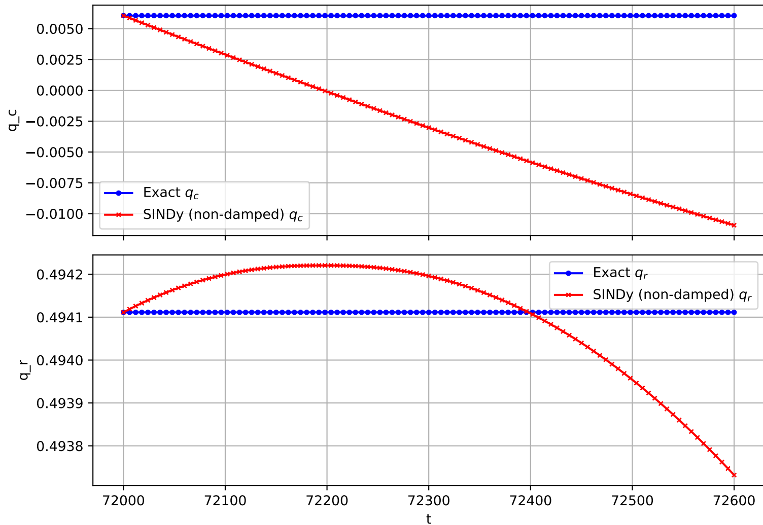
Trajectory 764 (non-damped)
