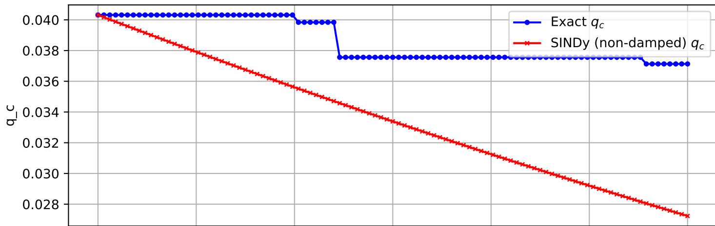
Trajectory 765 (non-damped)
