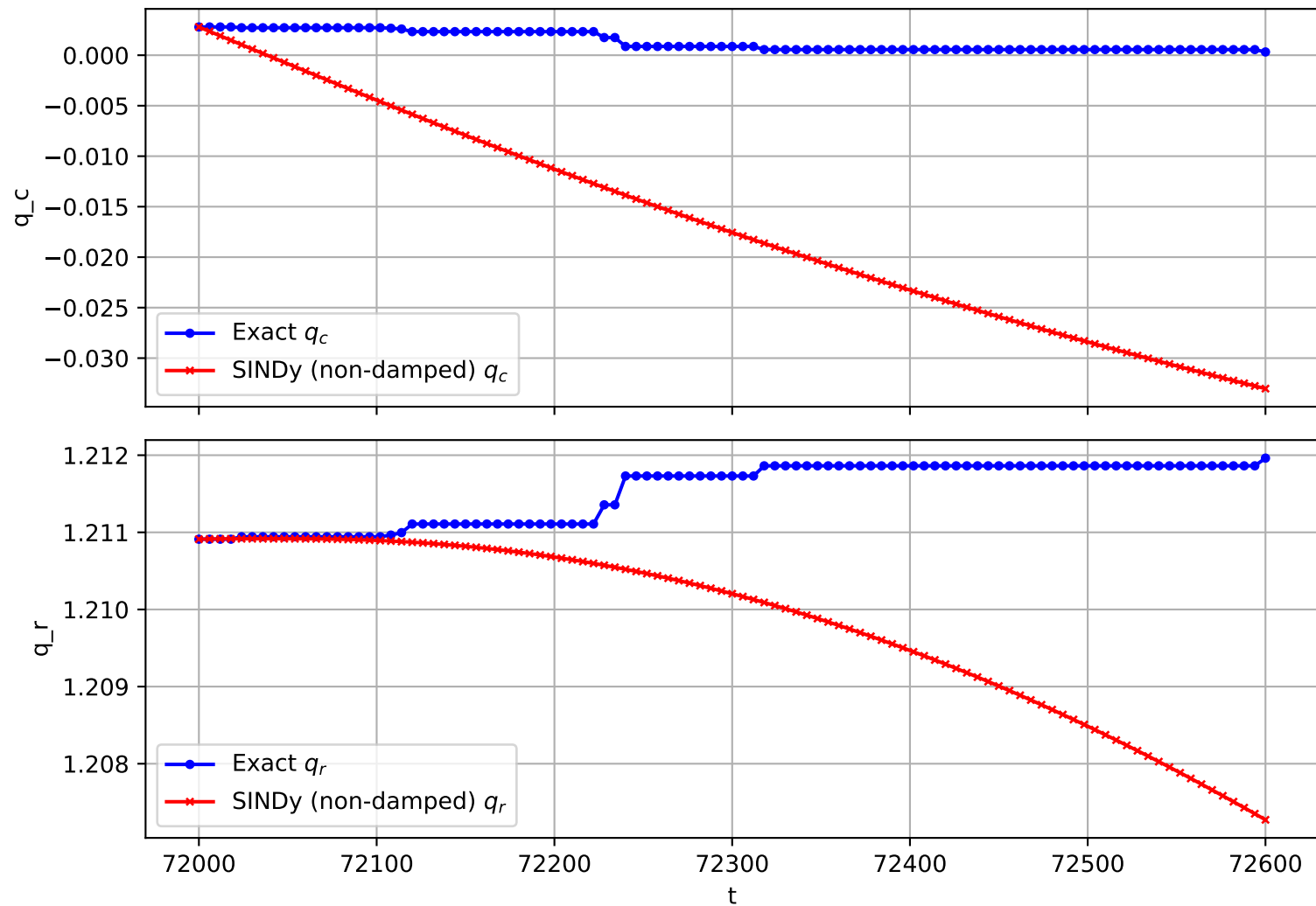
Trajectory 773 (non-damped)
