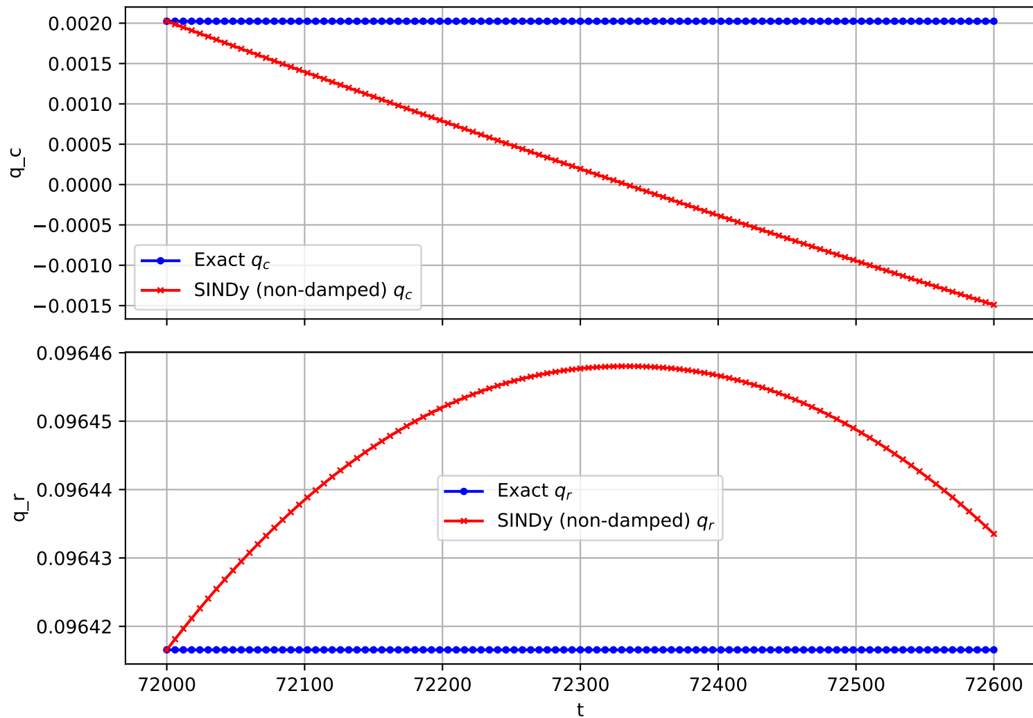
Trajectory 780 (non-damped)
