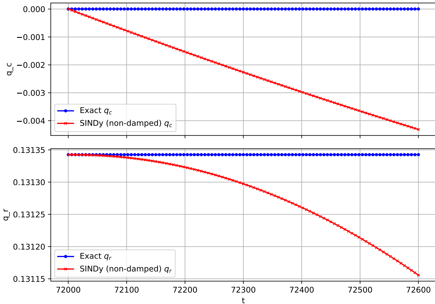
Trajectory 782 (non-damped)
