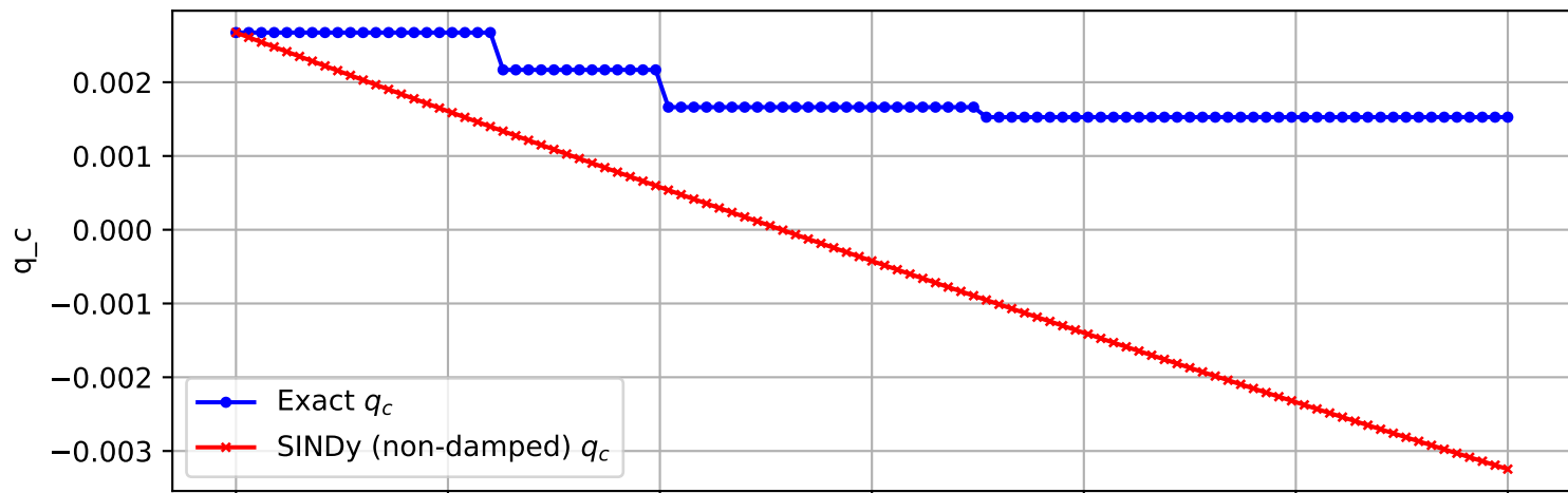
Trajectory 783 (non-damped)
