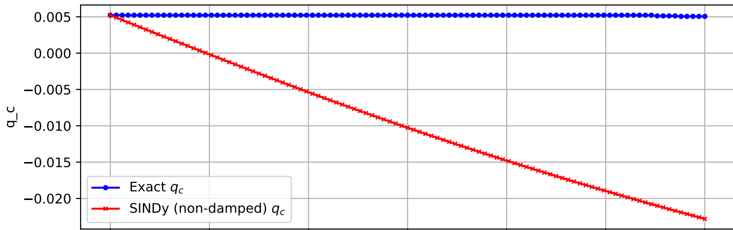
Trajectory 789 (non-damped)
