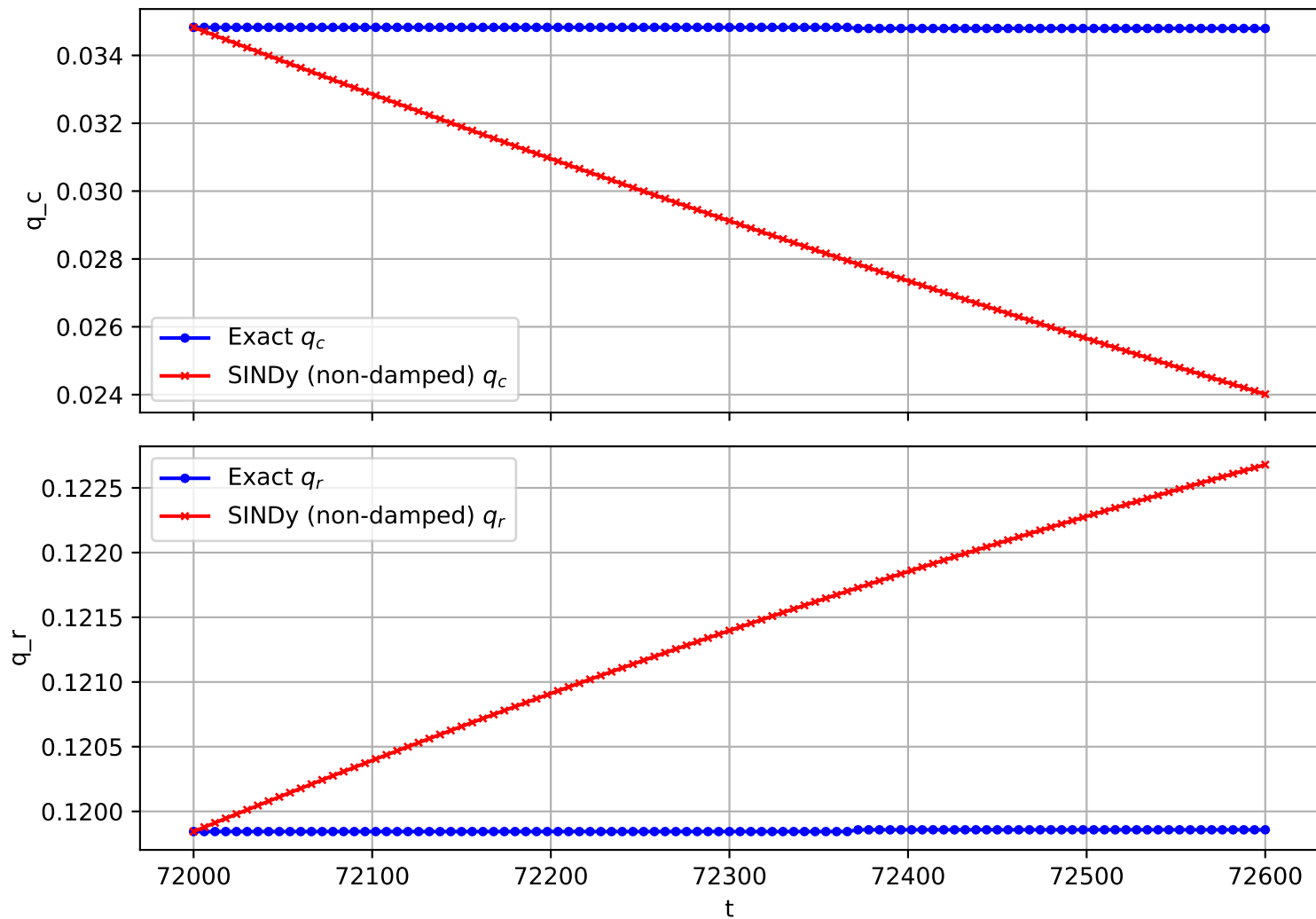
Trajectory 794 (non-damped)
