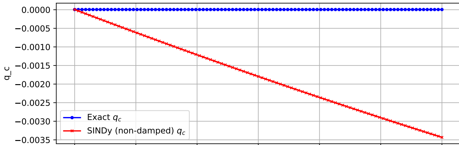
Trajectory 795 (non-damped)
