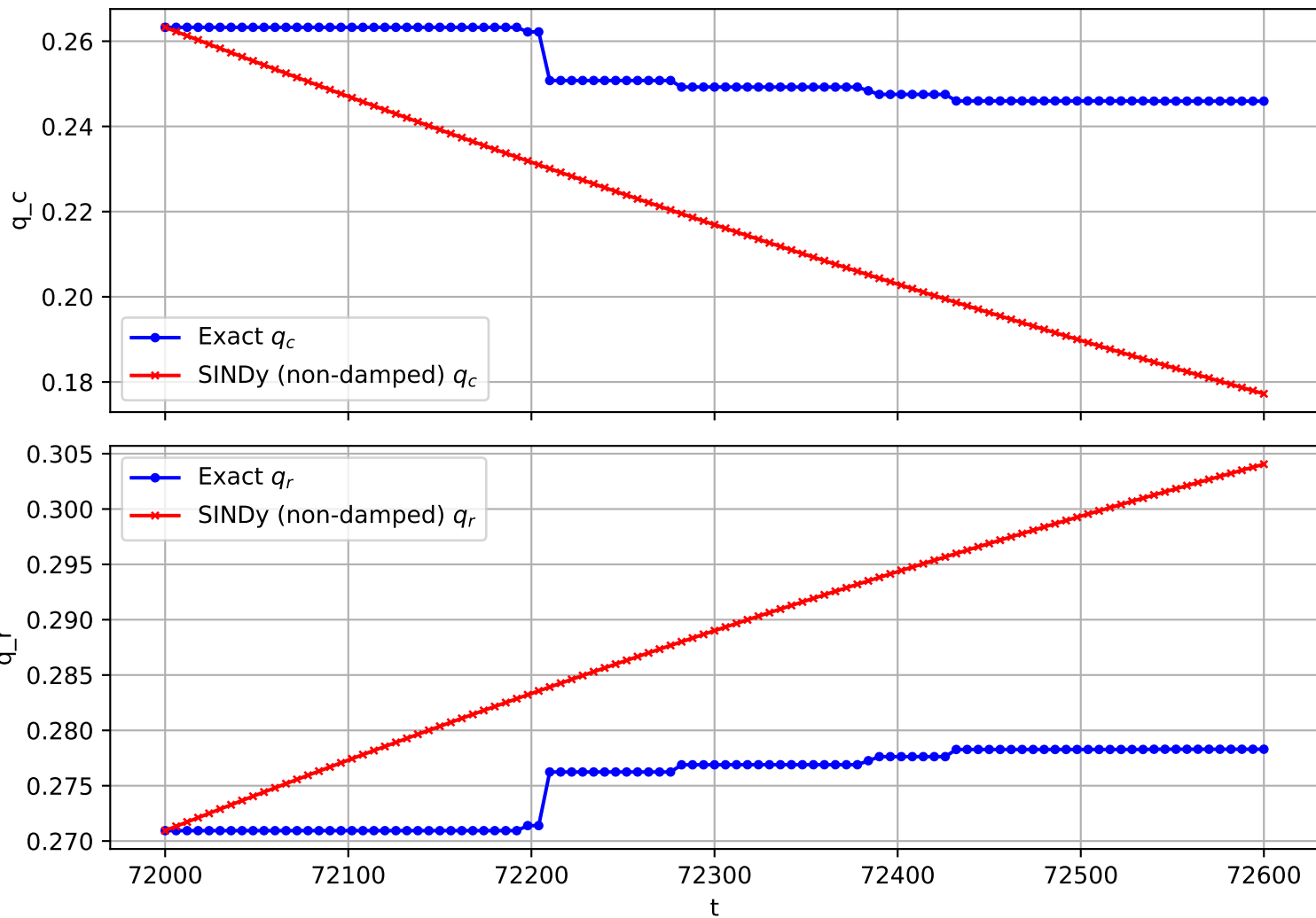
Trajectory 8 (non-damped)
