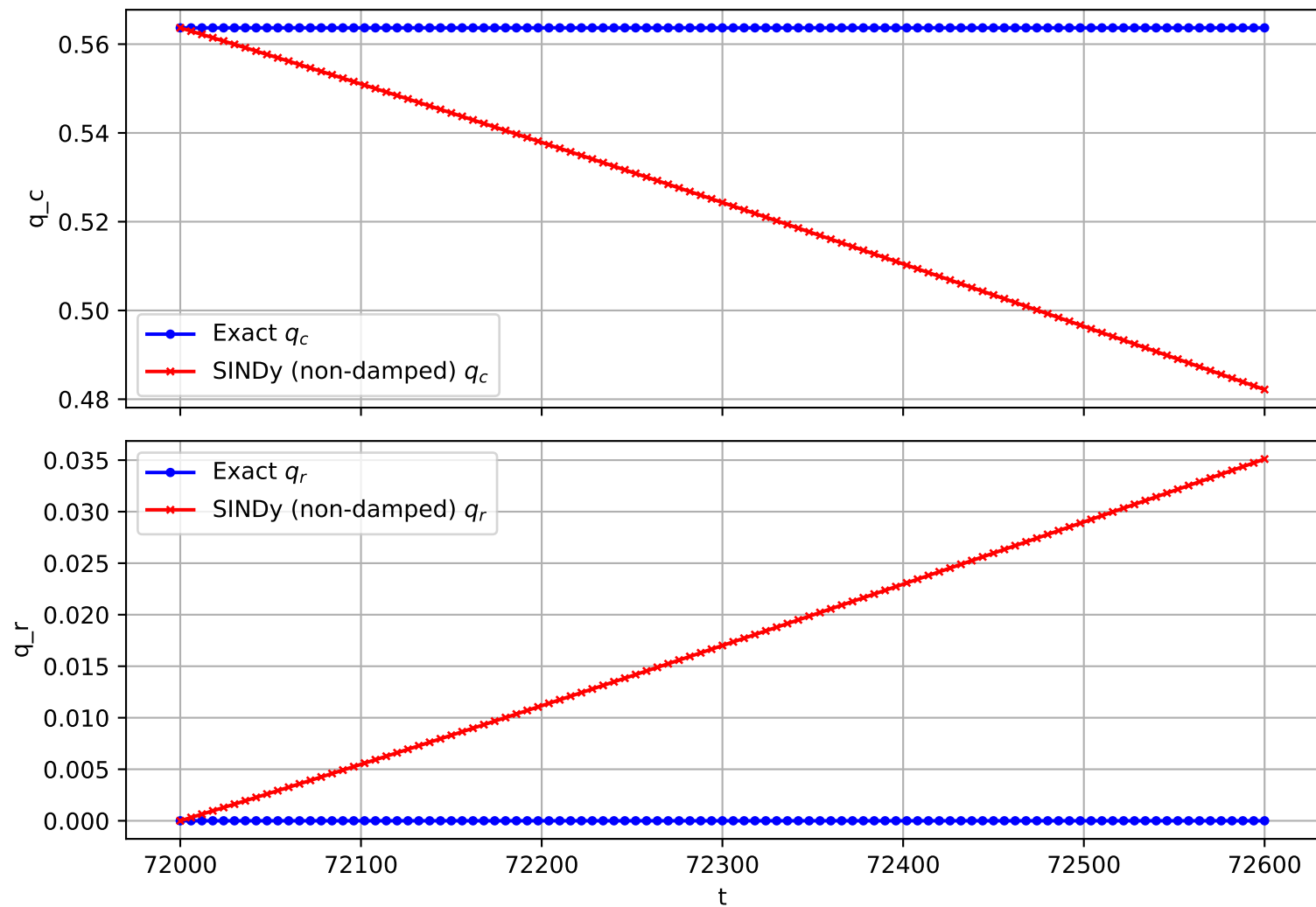
Trajectory 80 (non-damped)
