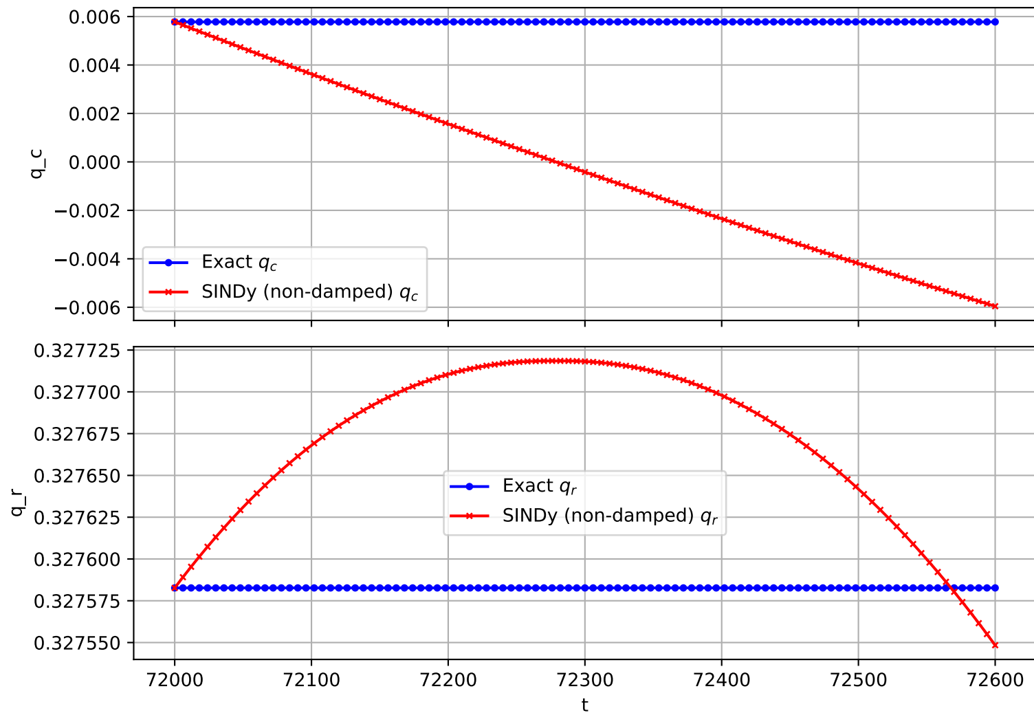
Trajectory 813 (non-damped)
