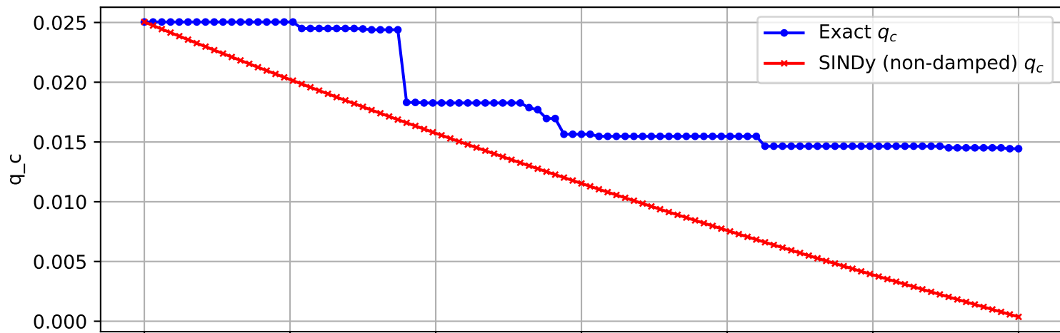
Trajectory 814 (non-damped)
