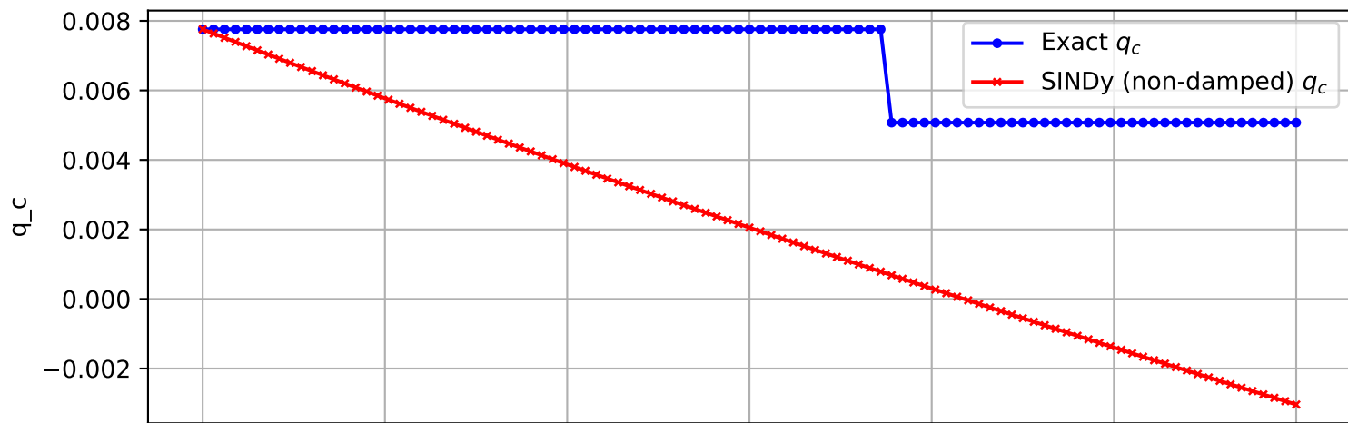
Trajectory 822 (non-damped)
