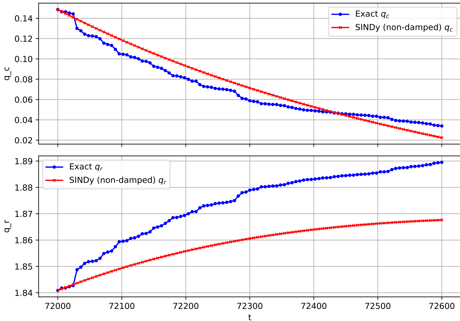
Trajectory 825 (non-damped)
