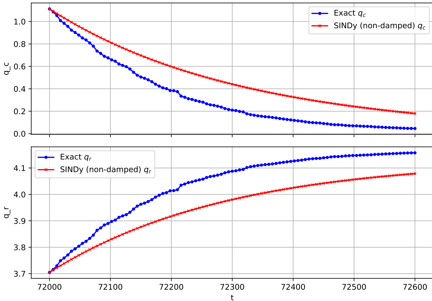
Trajectory 827 (non-damped)
