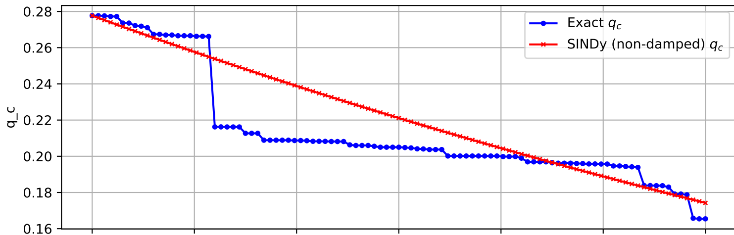
Trajectory 84 (non-damped)
