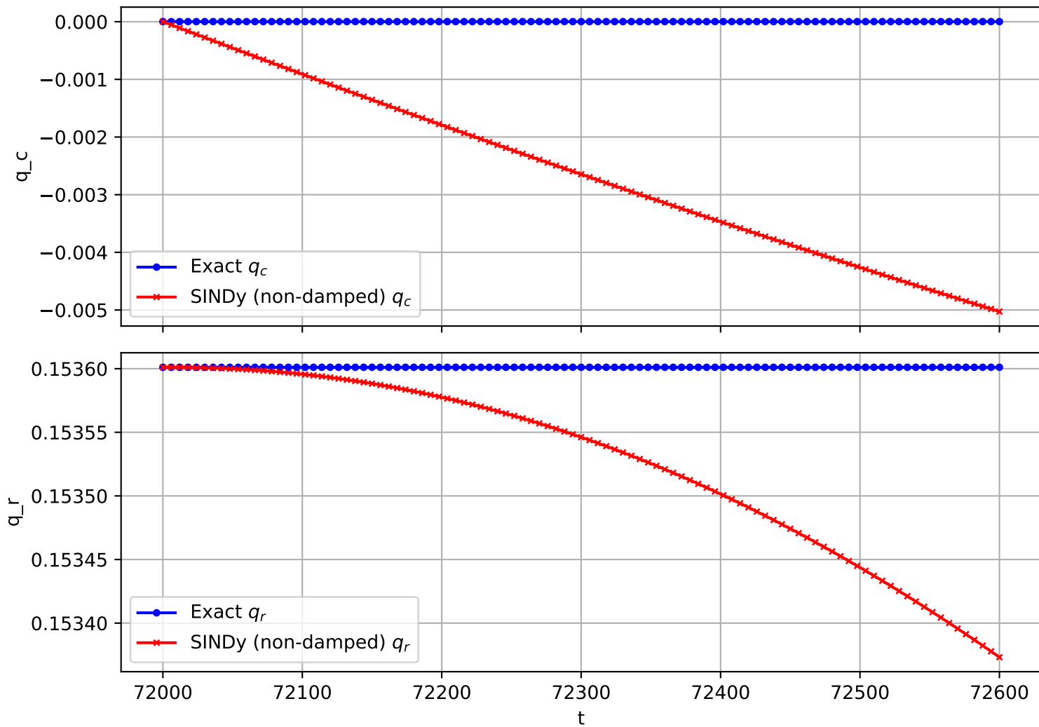
Trajectory 864 (non-damped)
