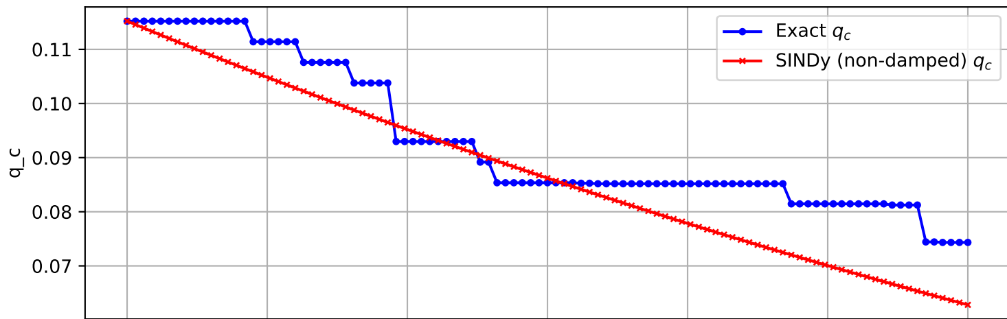
Trajectory 87 (non-damped)
