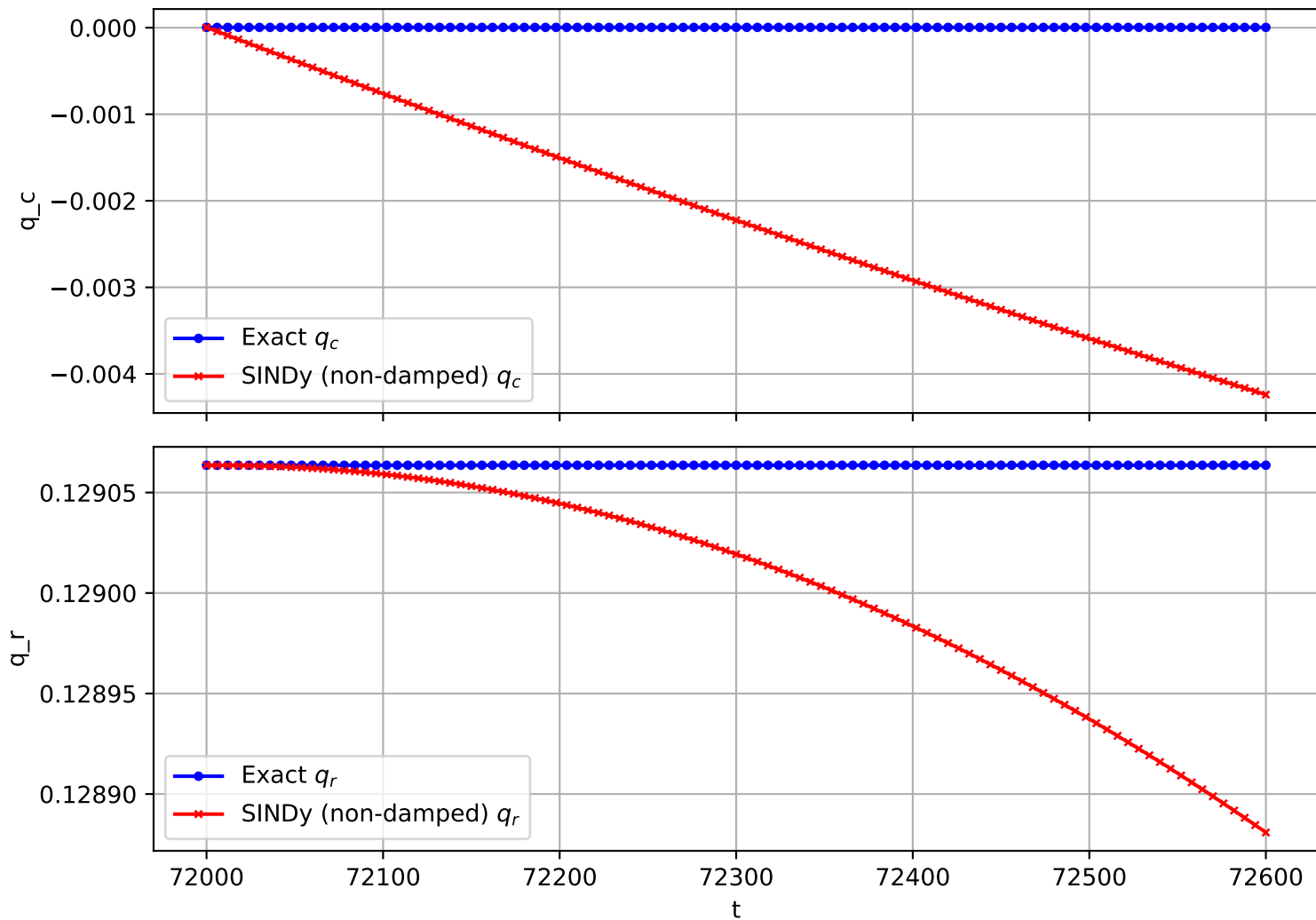
Trajectory 870 (non-damped)
