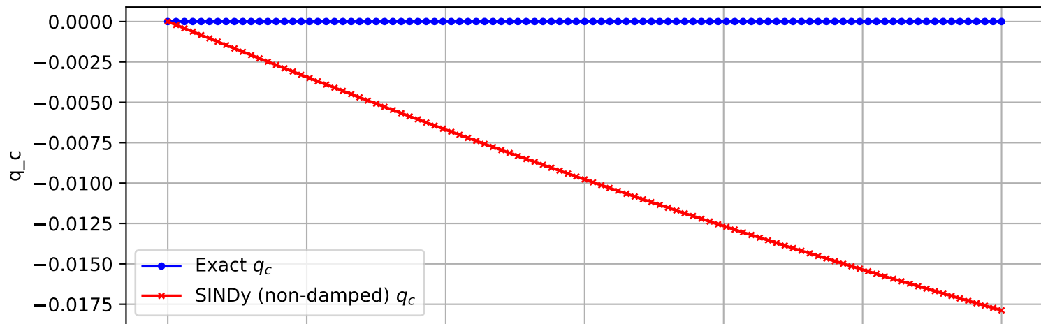
Trajectory 891 (non-damped)
