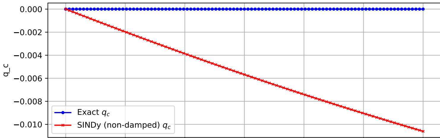
Trajectory 902 (non-damped)
