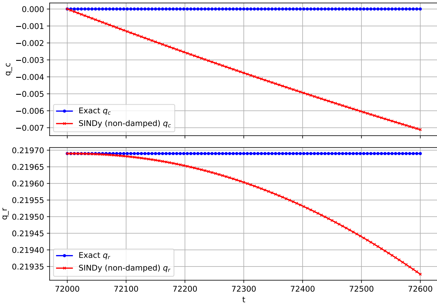
Trajectory 904 (non-damped)
