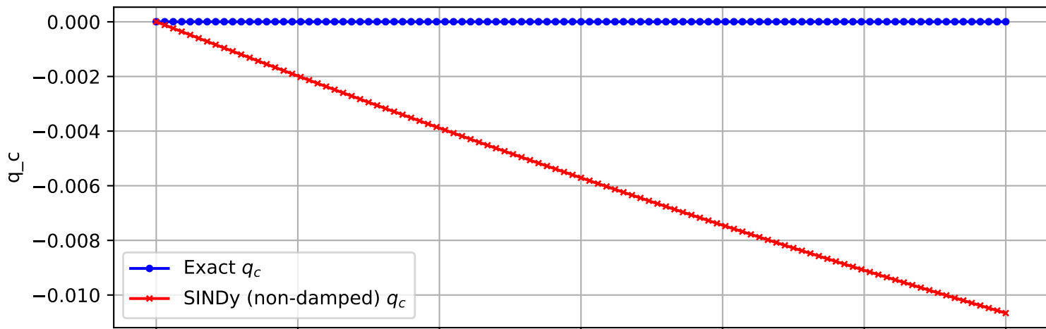
Trajectory 905 (non-damped)
